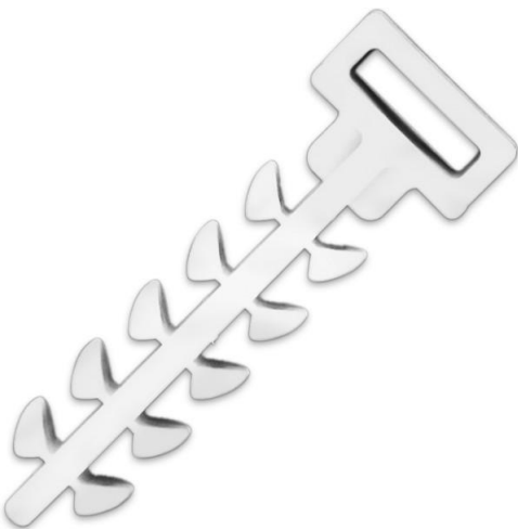
Steck-Dübel hellgrau, RAL7035, Bohrloch 6x27 mm, DIETZEL
