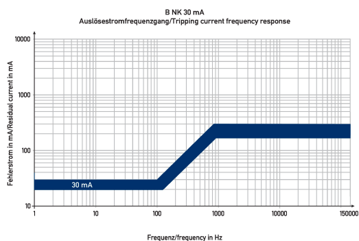
Diagramme FI-/LS-Kombinationen DRCBO 4 Co6/o,03/1N-B NK
