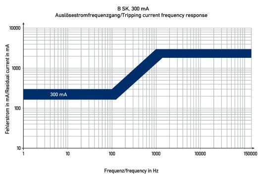
Diagramme FI-/LS-Kombinationen DRCBO 4 B25/0,30/1N-B SK
