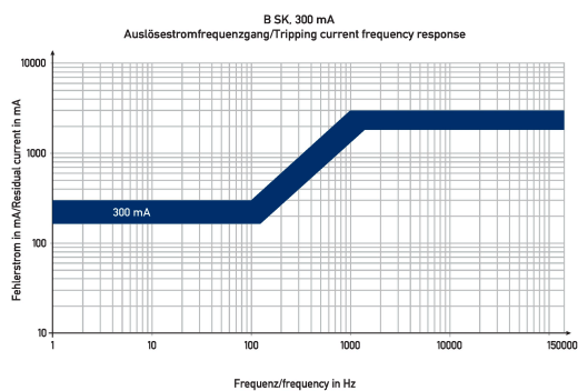
Diagramme FI-/LS-Kombinationen DRCBO 4 B16/o,30/1N-B SK
