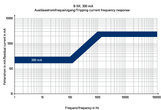
Diagramme FI-/LS-Kombinationen DRCBO 4 Bo6/o,30/1N-B SK
