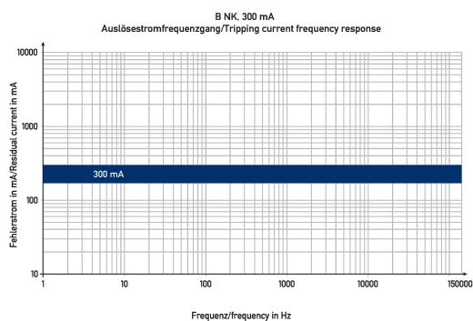
Diagramme FI-/LS-Kombinationen DRCBO 4 C16/0,30/3N-B NK
