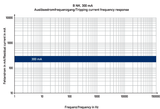
Diagramme FI-/LS-Kombinationen DRCBO 4 Co6/o,3o/3N-B NK
