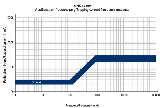
Diagramme FI-/LS-Kombinationen DRCBO 4 Co6/o,03/3N-B NK
