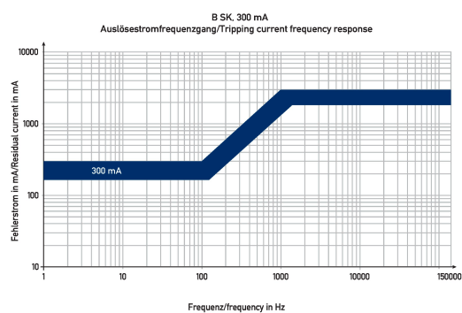
Diagramme FI-/LS-Kombinationen DRCBO 4 B25/0,30/3N-B SK
