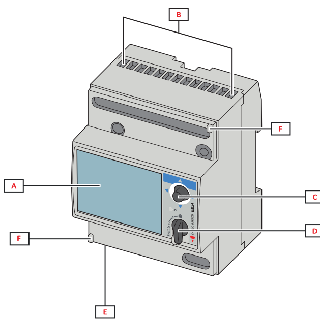
Fig. 2 CT connection
