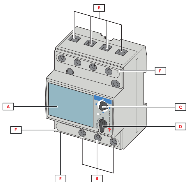
Fig. 1 Direct connection
