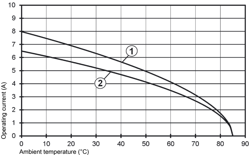
① Turned ② Stamped Conductor cross-section 0.75 mm²
