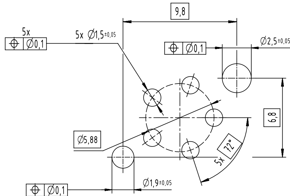
A (5:1) recommended PCB-layout
