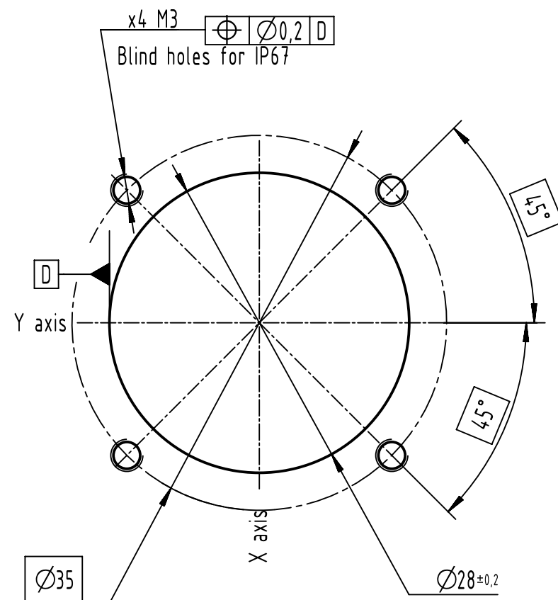
Panel cutting
