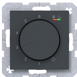
BERKER A.x/C.x Temp.regler 230V/15W, Heizen/Kühlen, anthrazit matt, lack.
