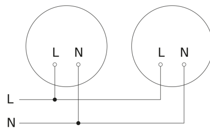
Schaltplan Master-Master Bluetooth
