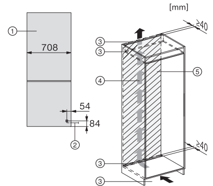
KFN7934D, Installation
