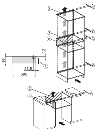
Installation EVS7010, Skizze
