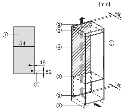
K7318D, K7328D, K7316E, K7326E, K7317D, K7327D, K7315E, K7325E, Installation (Fußnote*) (Skizze)
