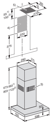
DAW1620, Skizze
