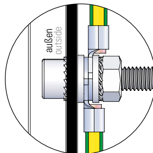
Variante 2: Anschluss innen variant 2: connection inside
