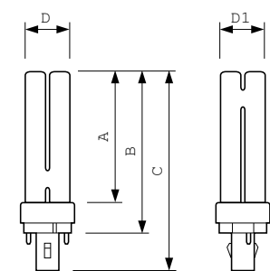
PL-C 18W/830/2P
